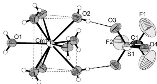
Figure 1. Structure of the [\text{An}(\text{H}_2\text{O})_9]^{3+} entity in 2 and 3 ( 3 is shown; thermal ellipsoids set at 40% probability) hydrogen-bonded to \text{CF}_3\text{SO}_3^- . The TTP geometry and hydrogen-bonding are indicated by dashed lines. Selected bond lengths [Å] for 2 , 3 , and 1 [3f] : Am–O1 2.578(6), Am–O2 2.466(4); Cm–O1 2.565(8), Cm–O2 2.454(6); Pu–O1 2.574(3), Pu–O2 2.476(4).
